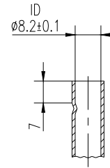
吐出管详细 DISCHARGE TUBE
