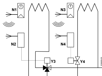
Zone valve
