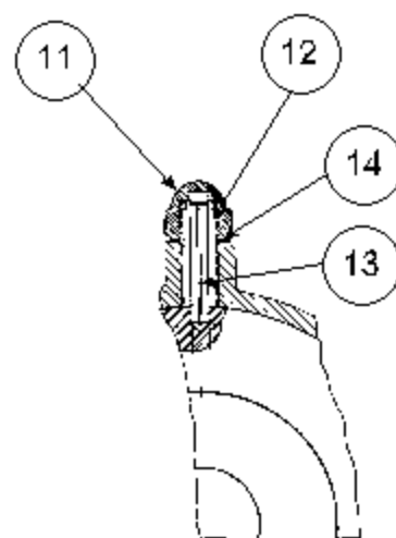
SECTION J-J
