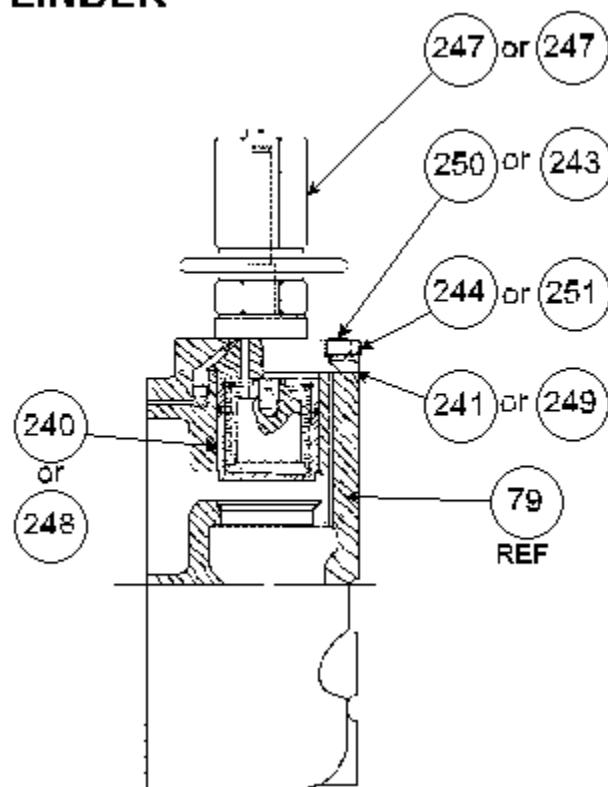
HOTGAS BYPASS CYLINDER HEAD
