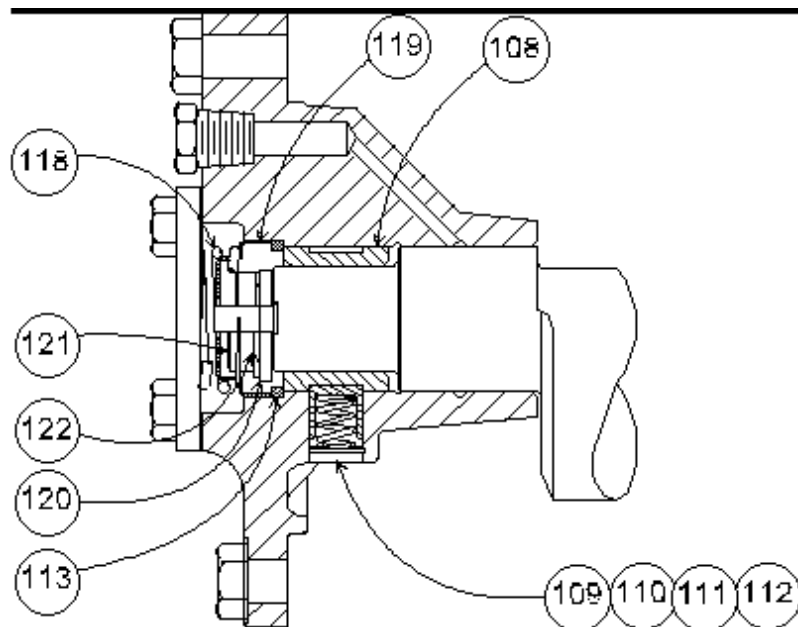
VIEW E-E from pgs 3,5,8
