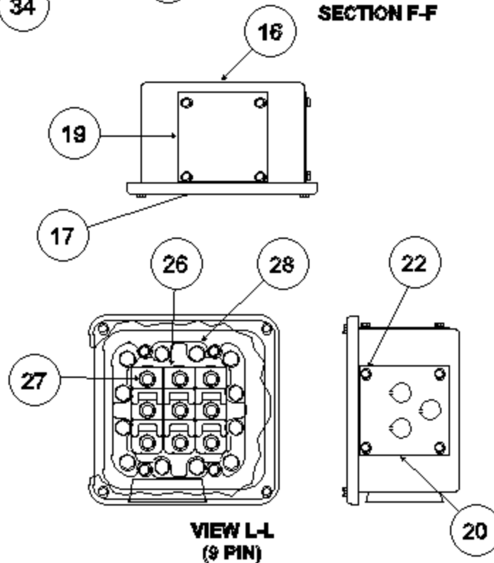
TERMINAL PLATE AND BOX CONFIGURATION FOR DUAL VOLTAGE CPRSRs
