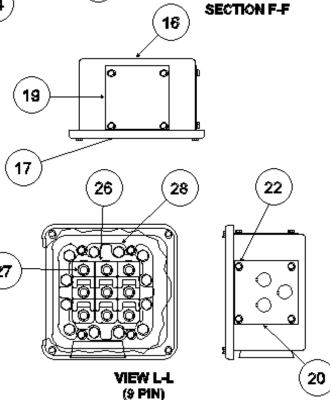
TERMINAL PLATE AND BOX CONFIGURATION FOR DUAL VOLTAGE CPRSRs
