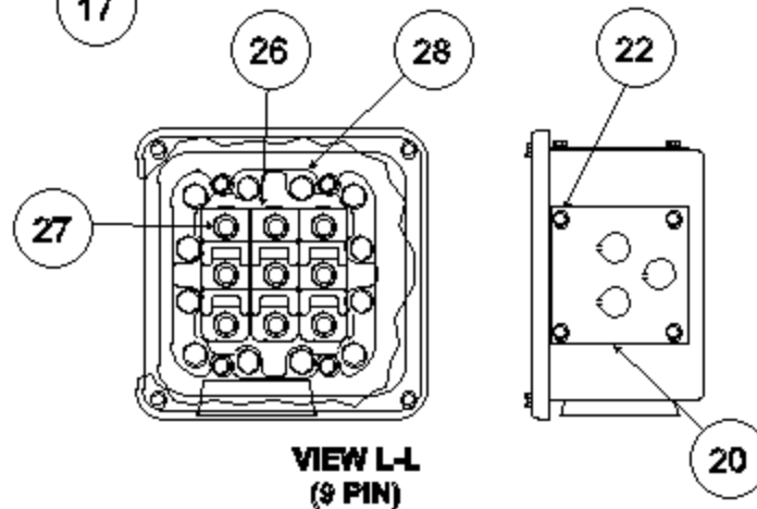
TERMINAL PLATE AND BOX CONFIGURATION FOR DUAL VOLTAGE CPRSRS
