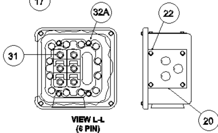
TERMINAL PLATE AND BOX CONFIGURATION FOR DISCRETE VOLTAGE CPRSRS
