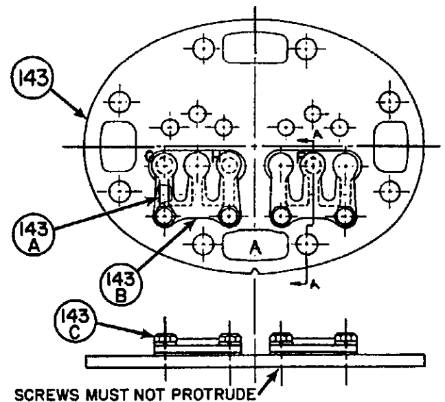
LOW STAGE VALVE PLATE, ITEM #120
