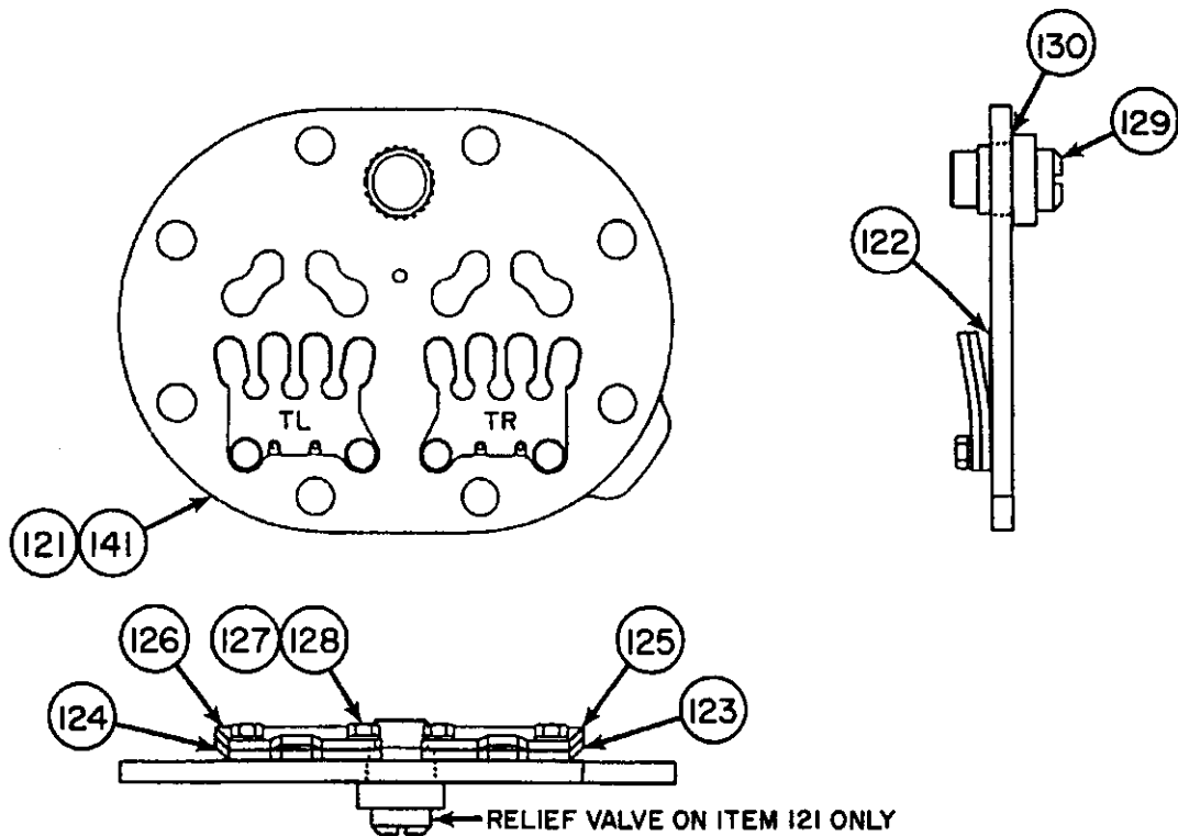
LOW STAGE VALVE PLATE
