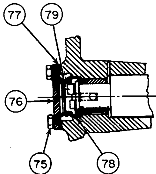
SECTION Q-Q
