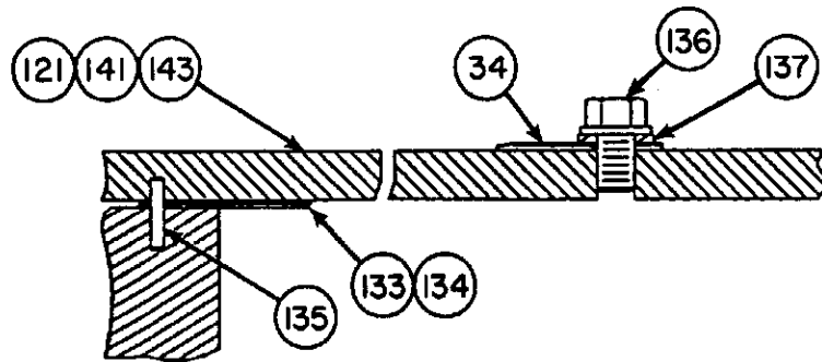
SECTION G-G
