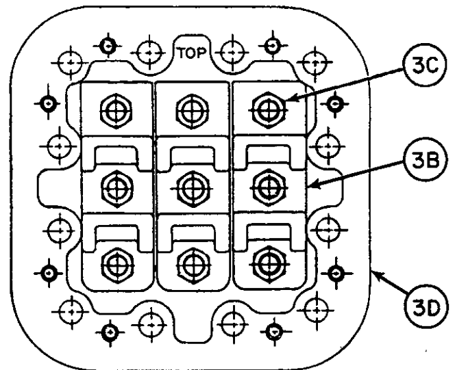
9 PIN TERMINAL PLATE FOR 208/230 PW & XL & 460/400 XL
