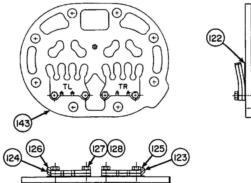
HIGH STAGE VALVE PLATE
