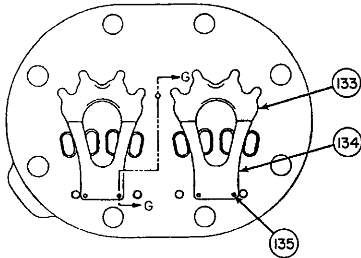
VALVE PLATE, CRANKCASE SIDE
