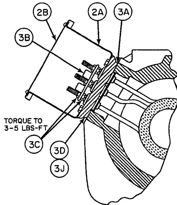
SECTION C-C
