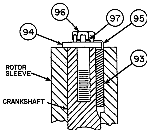
SECTION F-F
